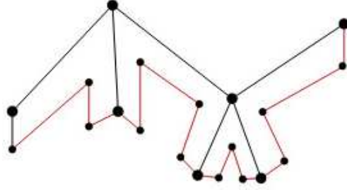
Figure 1: The path Q in the proof of Lemma 5.3.
