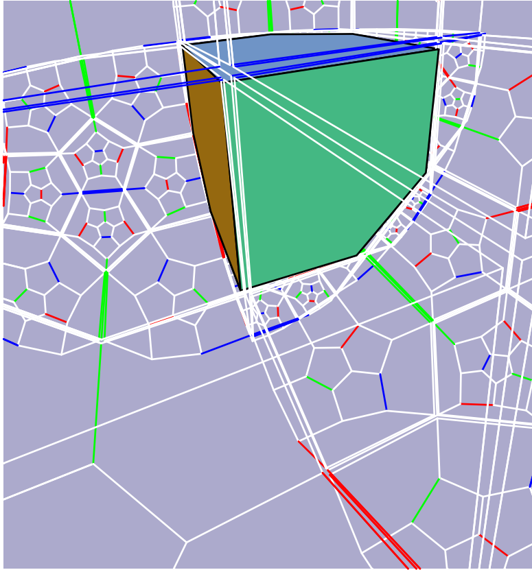
Figure 12. Hyperbolic space tiled by right-angled dodecahedra. This is a true perspective drawing inside T^3 when it has a hyperbolic metric with three singular axes of cone angle \pi . Compare with figure 11, frame 3. The fundamental domain (the dodecahedron) has many images, which appear in distorted perspective to Euclidean-adjusted eyes. The prominent circle is the horizon circle for one of the planar sheets of faces. Can you pick out any ‘bananas’, or rough hyperbolic cylinders, made from strings of dodecahedra? This figure is a postscript snapshot from geomview , a program available for common unix platforms from http://www.geom.umn.edu . Click on the Not Knot Flythrough module (written by Charlie Gunn) and you will be conducted on a flying tour through this scene (minus the solid dodecahedron). From the File menu open data/geom/dodec ; with patience you can translate and rotate dodec in one of the bays. Fancier versions of scenes like this occur in the video NotKnot .
