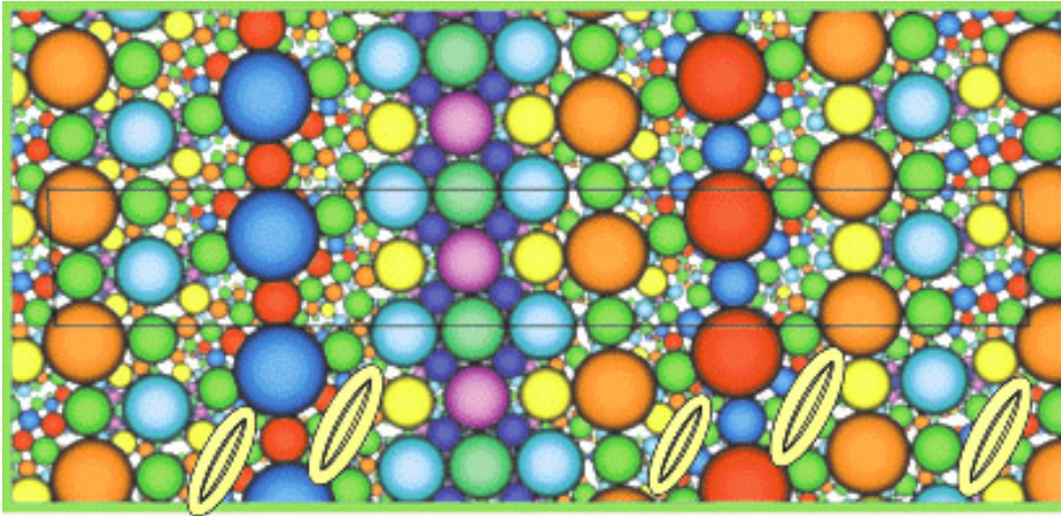
Figure 17. One of the cusp views of a nine-cusped hyperbolic manifold of volume 44.0227. The horosphere that walls off this cusp encloses a volume of 7.5; the next largest cusp volume is 4.2. Features that look like hyperbolic cylinders are scattered around the image, as indicated by the bananas sketched in at the bottom. Notice how the bananas together with the horoballs seem to fit in a semi-regular pattern, as for the cusp view for the Borromean rings but with dislocations where the grid turns 45^\circ . Patterns like this are common.
