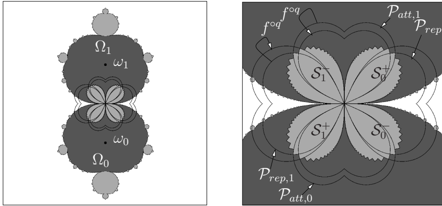
Figure 1: The parabolic basin of 0 for the polynomial P(z) = z + z^3 is colored grey. The parabolic multiplicity is 2. There are two attracting petals and two repelling petals. The connected components of the immediate basin are dark grey. The sepals are light grey.
