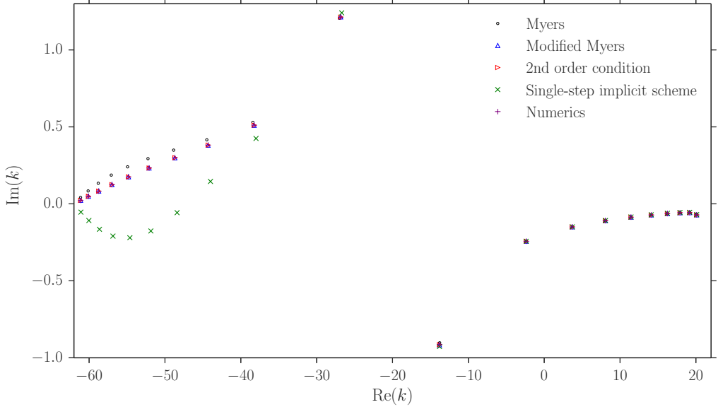
Figure 5. Least cutoff modes of the Myers condition (black circle), Modified Myers condition (blue triangle), single-step implicit scheme (4.11) (green cross), \mathcal{O}(\delta^2) asymptotic solution (3.8) (red right-triangle) and Pridmore-Brown numerics (purple plus), for \omega = 31 , m = 4 , M = 0.5 , \delta = 2 \times 10^{-3} and a tanh profile. The boundary impedance is Z_b = 3 + 4.61i .
