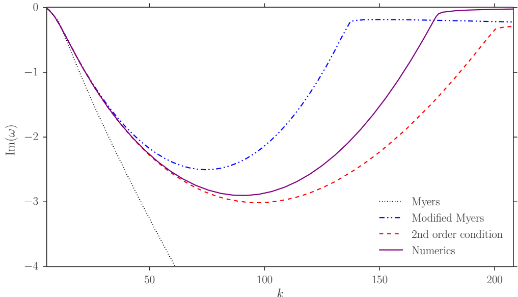
Figure 7. The unstable mode growth rate is plotted against real k for parameters \delta = 2 \times 10^{-3} , m = 12 , M = 0.5 , with a tanh boundary layer profile and a mass-spring-damper impedance, Z_b(\omega) = R + i\omega d - ib/\omega , for R = 3 , d = 0.15 , b = 1.15 , as in (7.1).
