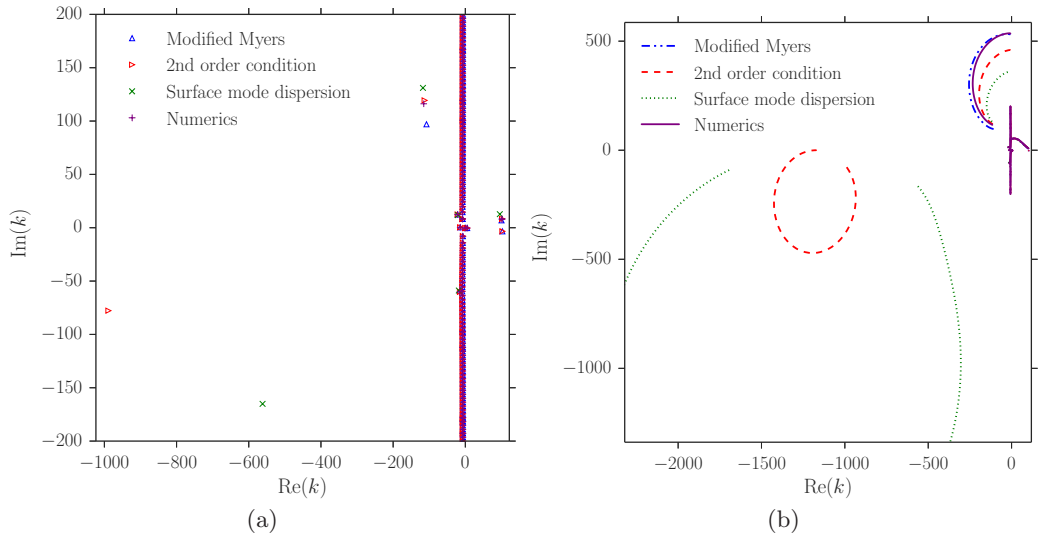
Figure 6. (a) Surface modes near the origin for Z_b = 1 - 2.5i , where here the mass-spring-damper model is not used. (b) A larger view of the k -plane, with tracks of surface modes as \text{Im}(Z_b) is increased from -2.5 with \text{Re}(Z_b) = 1 held constant. A spurious mode can be seen far from the origin. In both plots the parameters are \omega = 10 , m = 5 , \delta = 1 \times 10^{-3} , for a tanh profile with M = 0.5 .
