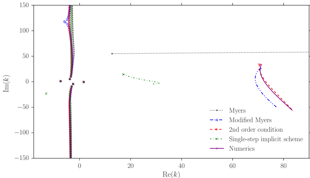
Figure 4. Modes in the k -plane of the Myers condition (black circle), Modified Myers condition (blue triangle), single-step implicit scheme (4.11) (green cross), \mathcal{O}(\delta^2) asymptotic solution (3.8) (red right-triangle) and Pridmore-Brown numerics (purple plus). The tanh boundary layer profile (6.1) is used, with a constant base density. Parameters are \omega = 5 , m = 0 , M = 0.5 , \delta = 2 \times 10^{-3} . The boundary impedance for the markers is Z_b = 3 + 0.52i . The lines track the surface mode for each boundary condition as \text{Im}(\omega) is reduced from zero to -10 , or sufficiently negative, as \text{Re}(\omega) is held constant, and the boundary impedance changes in line with (7.1).
