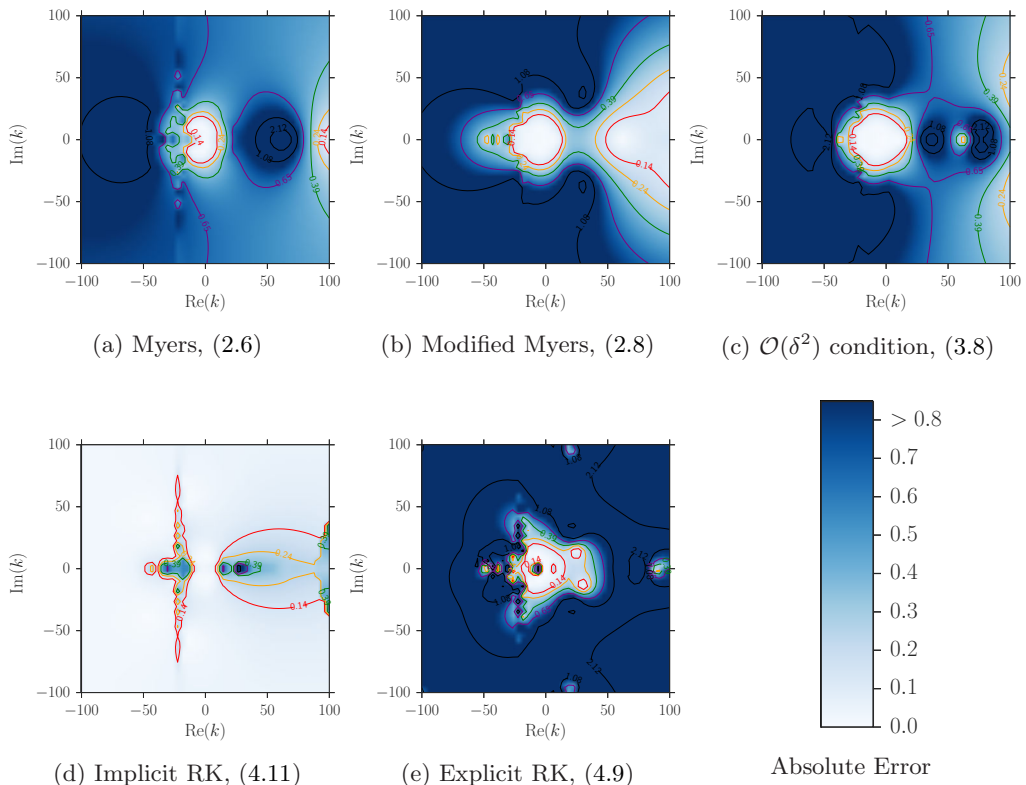
Figure 3. As in fig. 2, but for a boundary layer thickness \delta = 3 \times 10^{-2} . Note also the different error scale compared with fig. 2.
