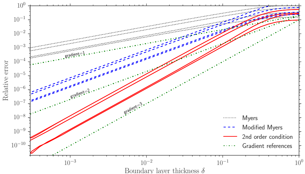
Figure 1. The relative errors of the leading (black dotted), first (blue dashed) and second (red solid) orders of the new boundary condition (3.8) when compared with numerical solutions of the Pridmore-Brown equation. The green dash-dot lines have gradients of 1, 2 and 3 beginning from the top and moving down. Parameters used are k = \pm 1 \pm i, \pm i and \omega = 1 , m = 0 , M = 0.5 with the tanh boundary layer profile of (5.1). Relative error is defined |Z^*/Z_{\text{eff}} - 1| , where Z^* is the approximation from the specified model, and Z_{\text{eff}} is the exact result from (2.7).
