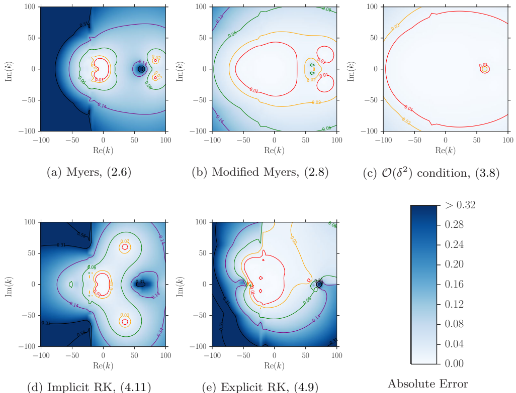
Figure 2. Absolute errors in the complex k -plane of the predicted Z_{\text{eff}} for each boundary condition. The colour scheme is normalised such that the darkest blue is an error greater than or equal to 1.5 times the mean Myers error. The red contour surrounds errors lower than the lowest quartile of the combined results for the Myers, Modified Myers, second order asymptotic and the single-step implicit Runge-Kutta conditions. Error was calculated as \min\{|Z_1 - Z_2|, |1/Z_1 - 1/Z_2|\} . Parameters are \omega = 31 , m = 24 , M = 0.5 , \delta = 2 \times 10^{-3} , for a tanh velocity profile (5.1) and constant base density \rho(r) \equiv 1 . The boundary impedance at each point is found from the numerical solution of the Pridmore-Brown equation, (2.3a).
