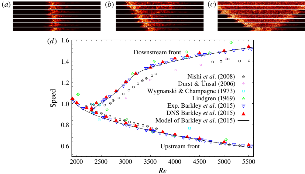
FIGURE 1. (Colour online) Temporal evolution of (a) a puff at Re = 2000 , (b) a slug at Re = 2600 , and (c) a slug at Re = 5000 . The flow is from left to right, and turbulence is visualised by the transverse turbulent fluctuations q (defined in § 2.1) in a frame of reference co-moving at the average of the upstream and downstream front speeds. The length scale in the vertical (radial) direction is stretched by a factor of 2 for better visualisation. Dark areas correspond to small fluctuations and bright areas correspond to large fluctuations. Time evolves in the upward direction and panels are separated by 10D/U in (a,c) and by 100D/U in (b), where U is the bulk velocity and D the pipe diameter. (d) Front speeds as a function of Reynolds number taken from the literature as indicated.
