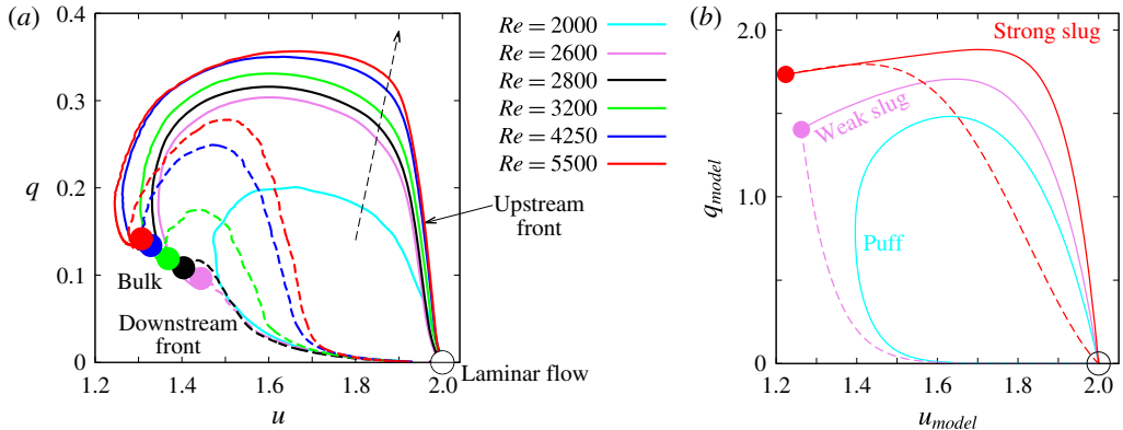
FIGURE 3. (Colour online) (a) The structure of turbulent–laminar fronts from DNS seen as trajectories in the (u, q) -phase plane. Upstream fronts for slugs are shown with solid lines while downstream fronts are shown as dashed lines. Filled circles correspond to the bulk region of the slug. The dashed arrow indicates the direction of increasing Reynolds number. The turbulent puff at Re = 2000 does not have a bulk region and for this case we do not distinguish upstream and downstream fronts with different line types. Trajectories form counterclockwise loops in the phase plane as one travels in space from the upstream to the downstream along the pipe. Phase-space trajectories have been obtained by averaging over time and over multiple runs at each Re (typically 20 runs with 150–500 snapshots per run, depending on Re ). (b) For comparison, the structure of turbulent–laminar fronts from a model of turbulent pipe flow (Barkley 2016). The trajectories are taken directly from Barkley (2016) figure 20.
