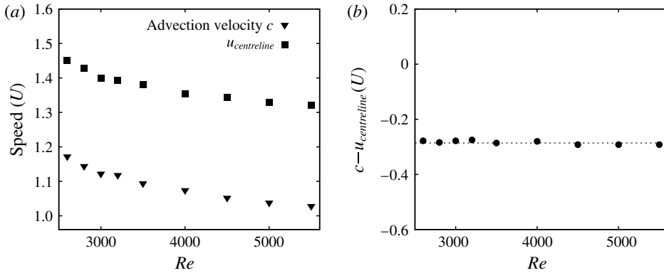
FIGURE 7. Comparison between the average turbulent advection speed and the average centreline velocity as a function of Re . (b) Difference between the advection speed and the centreline velocity.
