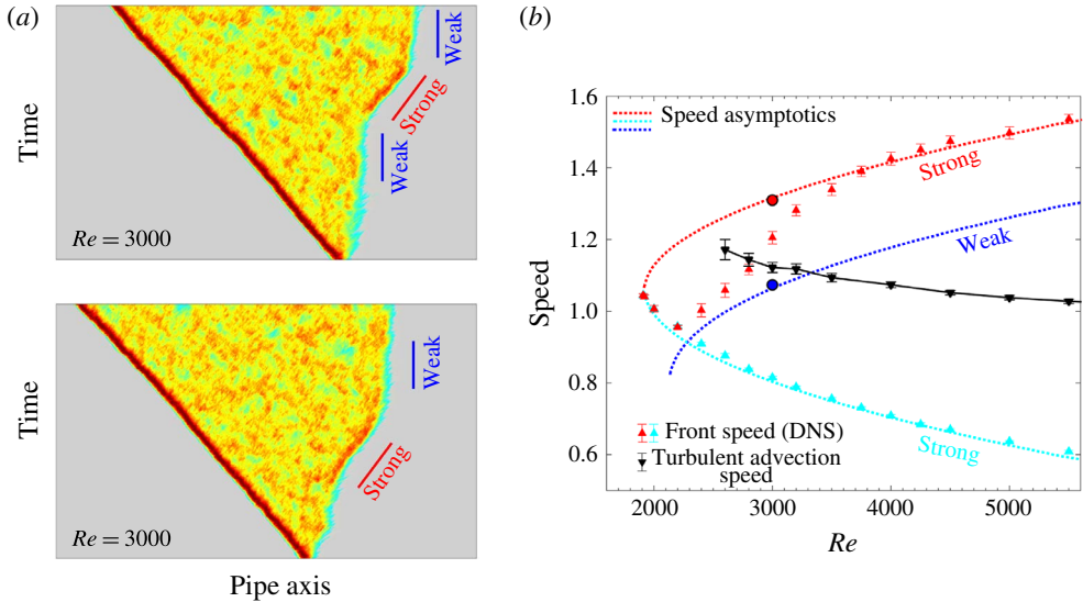
FIGURE 4. (Colour online) Switching between weak and strong front at Re = 3000 . (a) Space–time diagrams showing the colour map of q for two typical slugs in a moving frame of reference with the speed of 1.06U (the speed of the weak front at this Reynolds number). Grey areas correspond to small fluctuations and dark red areas correspond to large fluctuations. The bars show the slopes, i.e. the inverse of the speeds, of transient weak and strong fronts in this frame of reference. (b) Front speed as a function of Reynolds number from DNS (up-triangles) and from an asymptotic analysis of fronts in a model system (dotted lines), reproduced from Barkley et al. (2015). The circles show the speeds of the transient weak and strong fronts highlighted in (a). Black down-triangles show the mean turbulent advection speed in the bulk region of slugs computed using (4.2) and discussed in §4.
