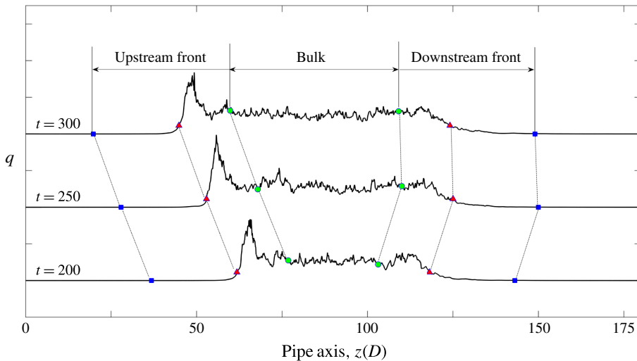
FIGURE 2. (Colour online) Division of a slug into upstream front, bulk and downstream front. A slug at Re=2800 is plotted at three time instants in a reference frame co-moving with the bulk flow. The flow is from left to right. Red triangles mark the position of the upstream and downstream fronts given by the cutoff q=0.02 . The bulk region is bounded between green circles, which are located 15D to the inside relative to the front positions (red triangles). Blue squares mark the beginning of the fronts and are located 25D to the outside relative to the front positions. With these choices the fronts span 40D in length.
