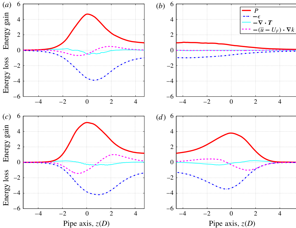
FIGURE 5. (Colour online) Kinetic energy budget (integrated over pipe cross-section) in the frame of reference co-moving with the fronts. Production (red bold line), dissipation (blue dash-dotted line), energy flux (cyan thin line) and convection (violet dashed line) are normalised by the mean turbulence production rate in the bulk. (a,b) Upstream front (UF) and downstream front (DF) of a slug at Re = 2600 . (c,d) Upstream front and downstream front of a slug at Re = 5000 . In (a,c,d) the peak of the production term is positioned at z = 0 . At each Reynolds number, an ensemble of about 500 snapshots is used to perform the energy budget analysis.
