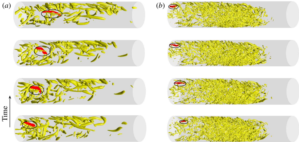
FIGURE 6. (Colour online) Advection of vortices near weak and strong fronts. (a) Weak front at Re = 2600 , (b) strong front at Re = 5000 . Vortices, visualised by using the \Lambda_2 criterion, are shown in the frame of reference co-moving with the downstream front (time evolves in the upward direction). The bulk turbulent region is on the left and the downstream laminar flow is on the right in the pipe. In each case one vortex is highlighted by red colour and a circle and is tracked in time. In (a) the time separation between two consecutive panels is 1.5D/U , whereas in (b) it is 0.625D/U .
