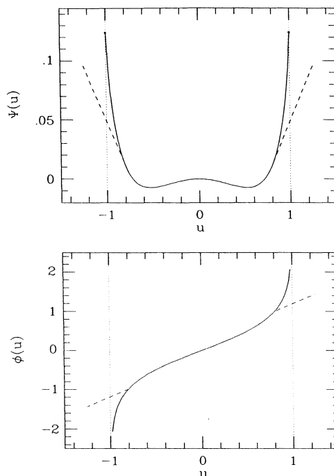
Fig. 1. The solid lines represent \Psi and \phi and the broken lines represent \Psi_\varepsilon and \tilde{\phi}_\varepsilon
