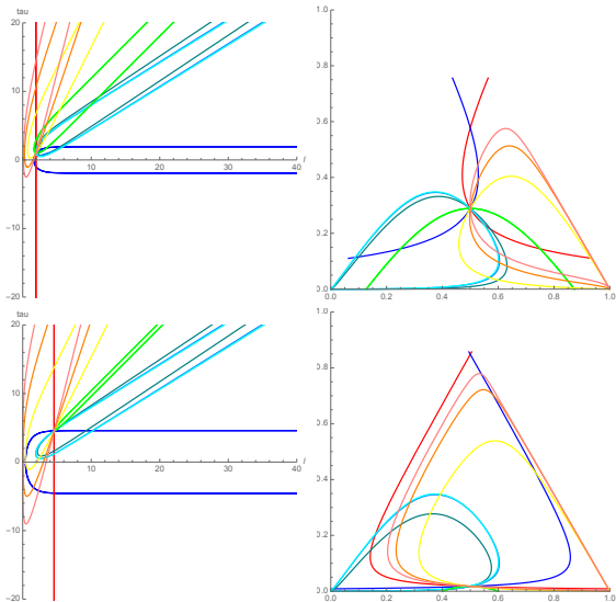
Figure: More example earthquakes in Fenchel-Nielsen coordinates (left) and on the simplex (right) with different starting across top and bottom.
