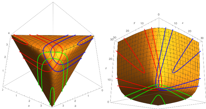
Figure: Example earthquakes about \alpha , \beta , \alpha\beta in triangle lengths (left) and trace coordinates (right) with different starting points.
