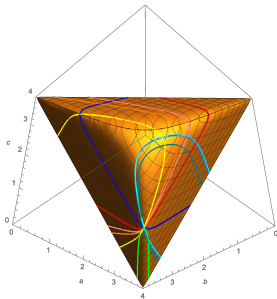
Figure: More example earthquakes in triangle lengths (left) and trace coordinates (right) with different starting across top and bottom.
