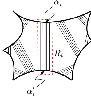
FIGURE 6. The rectangle R_i \subset D is surrounded by the dotted line. The arc \alpha_i in \partial D \cap X is indicated. In general the arc \alpha'_i may lie in X or in Y .
