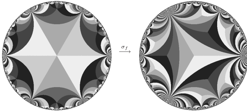
Figure 3.2. The pullback map \sigma_f fixes 0. It sends hexagons to triangles. There is a critical point with local degree 2 at the center of each hexagon and a corresponding critical value at the center of the image triangle. The map X \circ A sends light grey hexagons to the unit disk in \mathbb{P}^1 - \Theta and dark grey hexagons to the complement of the unit disk in \mathbb{P}^1 - \Theta . The map \pi sends light grey triangles to the unit disk in \mathbb{P}^1 - \Theta and dark grey triangles to the complement of the unit disk in \mathbb{P}^1 - \Theta .
