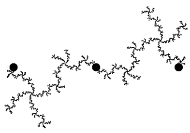
Figure 4.3. The Julia set of the degree 4 polynomial f : z \mapsto 2i(z^2 - \frac{1+i}{2})^2 is a dendrite. There is a fixed critical point at \infty . Its basin is white. The point z = 1 is a repelling fixed point. All critical points are in the backward orbit of 1.
