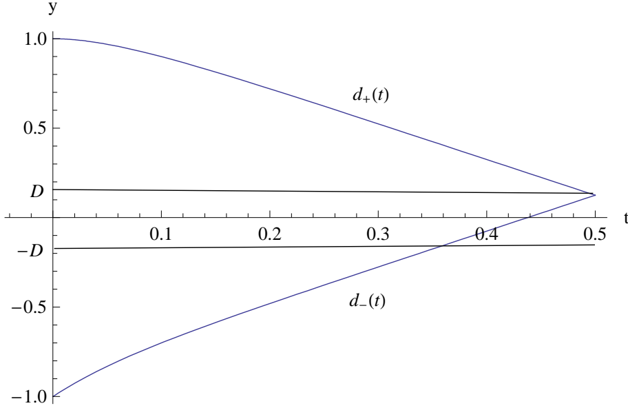
Figure 1: When the chain is pulled sufficiently fast, the process y_t is unlikely to leave the corridor of width D = d_+(b/a - 1) , so must hit d_-(t) first (shown here for U(y) = y^2 - 4y + 3 and \varepsilon = 0.25 ).
