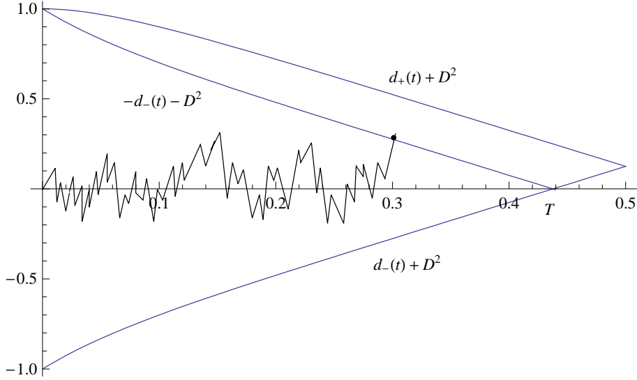
Figure 2: When the chain is stretched slowly, we show that conditional probability of hitting the curve d_+(t) + D^2 before d_-(t) + D^2 , when started from -d_-(t) - D^2 , goes to one as \sigma \downarrow 0 .
