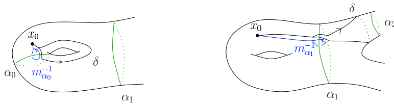
Figure 2. Homotopy classes of meridians.
