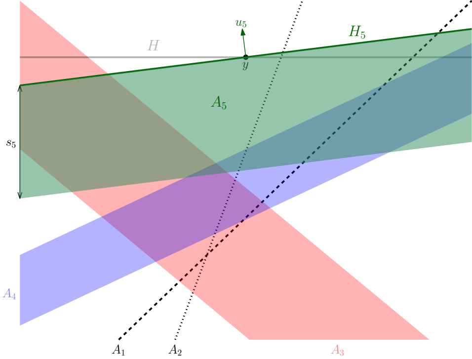
Figure 2: A_5 is obtained by modifying A . It satisfies (i), (ii), (iii), and (iv).
