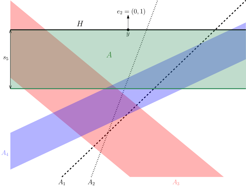
Figure 1: If A = A_{k+1} then conditions (ii), (iii), and (iv) hold.
