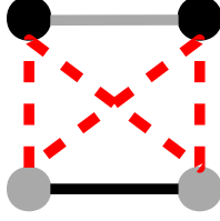
Figure 1: A feasible colouring of K_4 with respect to (C_5, C_5, C_5) , with two different colours on vertices
