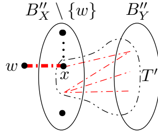
Figure 3: Finding a copy of T \in G_1 .
