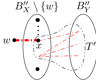
Figure 3: Finding a copy of T \in G_1 .
