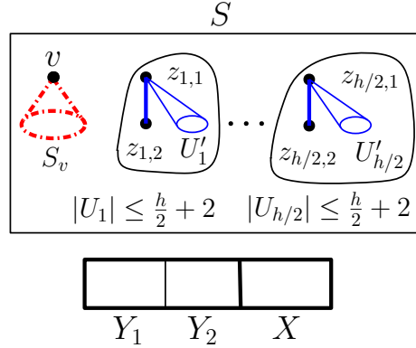
Figure 2: Case 2 of Lemma 3.2
