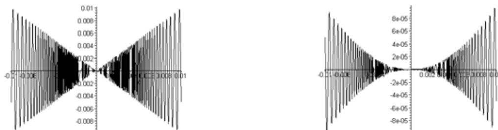
Figure 3: The curves y = x \sin(1/x) and y = x^2 \sin(1/x) .
