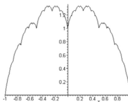
Figure 3: The blancmange.
