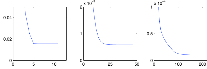
FIG. 4.10. Plots of \mathcal{J}_h(\underline{a}^k) for L = 5 (left), L = 10 (centre) and L = 25 (right) with y_T given by (4.18).
