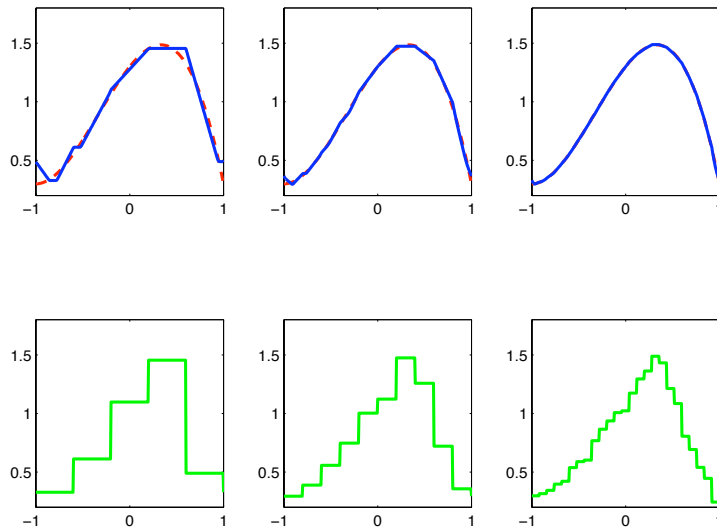
FIG. 4.2. Results for (4.19), upper plots show Y^T (dashed line) and Y_a^N (solid line), lower plots show \underline{a} .
