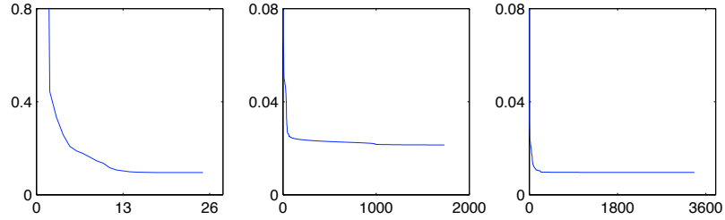
FIG. 4.12. Plots of \mathcal{J}_h(\underline{a}^k) for L = 5 (left), L = 10 (centre) and L = 25 (right) with y_T given by (4.23).
