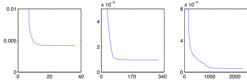
FIG. 4.11. Plots of \mathcal{J}_h(\underline{a}^k) for L = 5 (left), L = 10 (centre) and L = 25 (right) with y_T given by (4.20).
