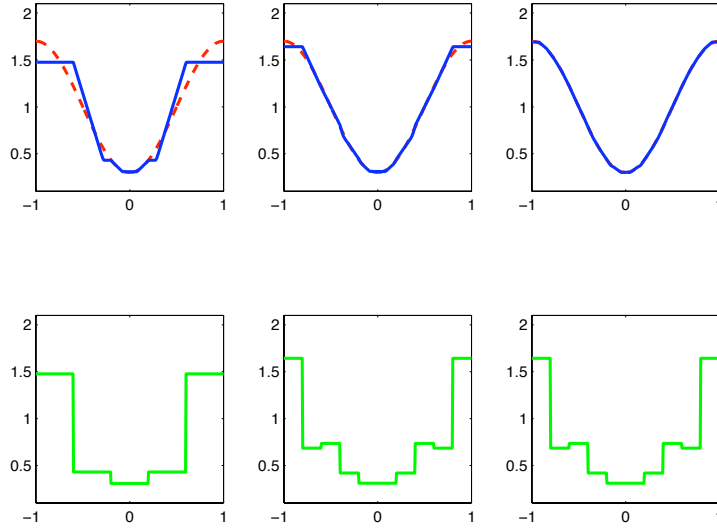
FIG. 4.1. Results for (4.18), upper plots show Y^T (dashed line) and Y_a^N (solid line), lower plots show \underline{a} .
