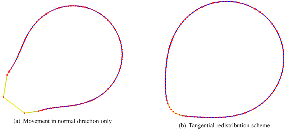
FIGURE 2. (Online version in colour.) Snapshots of the mesh during two simulations of cell motility using a scheme that moves the nodes only in the normal direction and the scheme that includes a tangential velocity. The large deformations result in meshes that are not suitable for computation with the former approach necessitating a remeshing step while with the latter approach the mesh quality remains good throughout.
