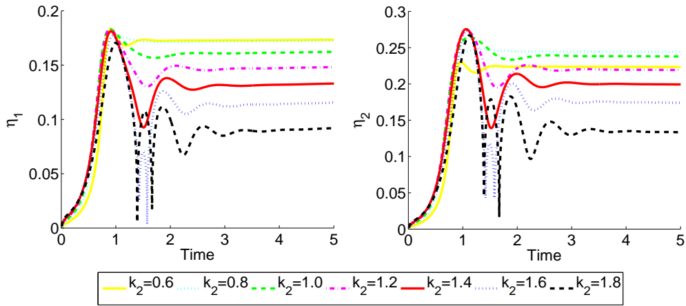
FIGURE 12. (Online version in colour.) Asymmetry measures vs. time of the cells shown in Figure 10. We observe larger deviations from reflection symmetry in the cells travelling at slower speeds. As the cells attain persistent shapes the values converge to a steady state.
