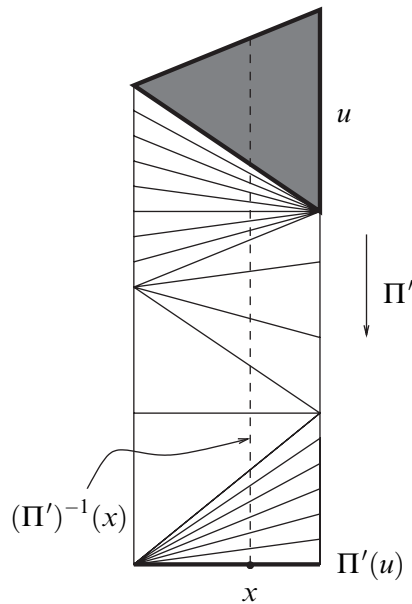
Figure 2. The deformation retraction above a simplex \Pi'(u) .
