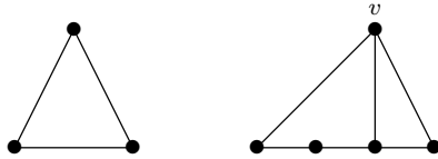
Figure 5: Evasive and non-evasive spherical graphs.
