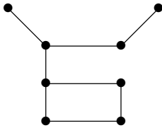
Figure 1: A graph with a two-element core.
