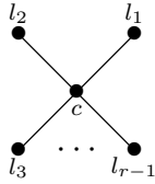
Figure 4: A star.
