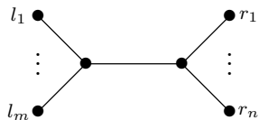
Figure 2: The conical tree T_{m,n} .
