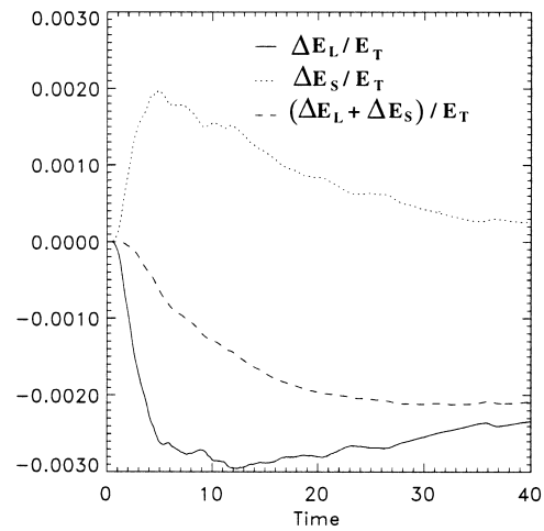
Fig. 21. Decaying turbulence with the interaction term switched off: small-scale energy E_S/E_T , variations in the large-scale energy \Delta E_L/E_T and the error (\Delta E_L + E_S)/E_T (run 7 without the interaction term).
