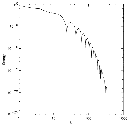
Fig. 29. Initial energy spectrum in the vortex merger problem, runs 8, 12 and 13.
