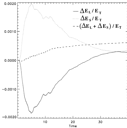
Fig. 20. For run 7, decaying turbulence: small-scale energy E_S/E_T , variations in the large-scale energy \Delta E_L/E_T and the error (\Delta E_L + E_S)/E_T (run 7).
