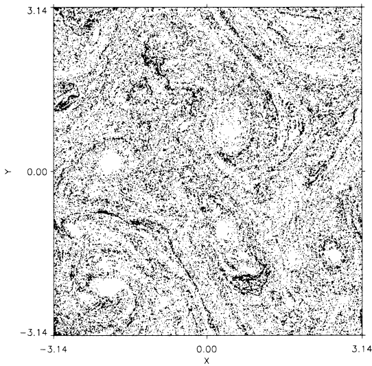
Fig. 6. Position of the same 50 000 particles as in Fig. 5 at t = 25 . After a long time, particles are mixed by turbulence except at the vortex cores (run 2).
