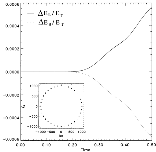
Fig. 16. Variations in the small-scale and large-scale energies, (\Delta E_S/E_T) and (\Delta E_L/E_T) in the case of initially isotropic small scales ( E_T = E_L + E_S ) (run 5). Insert shows the initial particle distribution in the wave number space.
