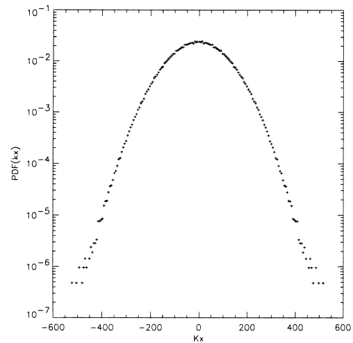
Fig. 11. For run 2, distribution of particles on the k_x axis at t = 0 (Gaussian distribution with \sigma = 100 ).
