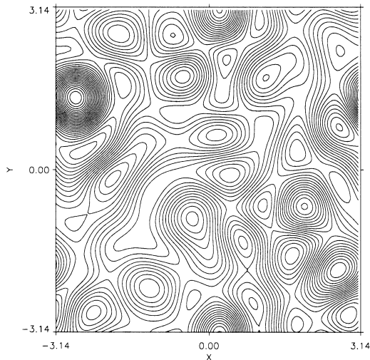
Fig. 18. Stream function of the large-scale vorticity field at t = 0.2 for run 6.
