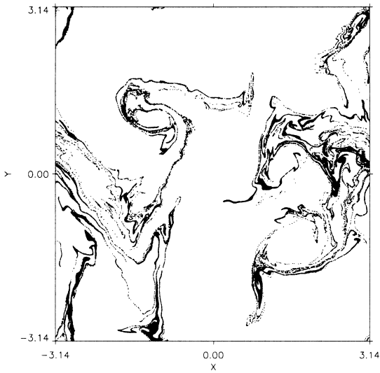
Fig. 5. Coordinates of 50 000 particles initially located in a strip -\pi \leq x \leq -\pi + \delta x shown at time t = 5 (run 2).
