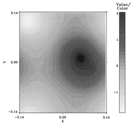
Fig. 8. Large-scale stream function at t = 50 for run 2. Small vortices have merged into bigger ones and the large-scale field has become essentially anisotropic.
