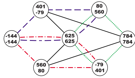
FIG. 6. (Color online) Example of a nontrident cluster of length 4. Wave numbers m, n are shown in the circles as upper and lower numbers. Solid black, dashed blue, dotted-dashed red, and dotted green lines connect the wave vectors forming first, second, third, and fourth quartets of the cluster correspondingly.
