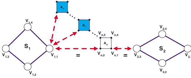
FIG. 7. (Color online) Schematic presentation of mixed resonance cascade.
