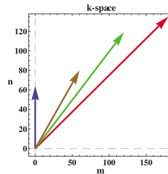
FIG. 4. (Color online) Wave vectors are shown which form first nontrident (nontrident with the smallest possible wave numbers m, n ).
