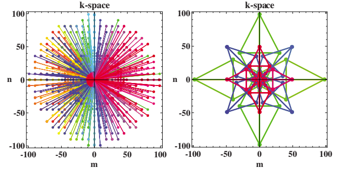
FIG. 2. (Color online) Structure of collinear resonances in the spectral domain m, n such that |\mathbf{k}| = |\sqrt{m^2 + n^2}| \leq 100 (left-hand panel) and of noncollinear resonances in the same domain (right-hand panel). Wave vectors belonging to different resonance quartets are shown in different colors.
