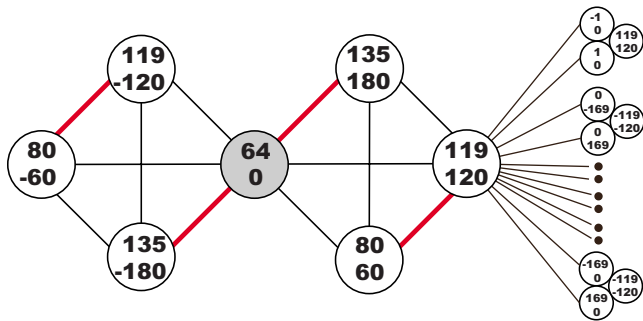
FIG. 8. (Color online) Wave numbers m, n are shown in the circles as upper and lower numbers. Wave (64, 0) takes part in two scale resonances, both nontridents. The upper number in the circle is m , the lower is n , and (red) thick lines drawn between vectors on the same side of Eqs. (3). Wave (119, 120) takes part in one scale resonance and in 12 angle resonances.
