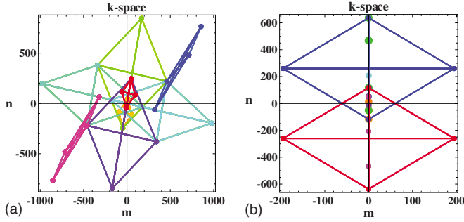
FIG. 5. (Color online) Wave vectors belonging to one resonant quartet are depicted in the same color. Left-hand panel: A shortest cluster formed by both tridents and nontridents; cluster length is 8 (64 with eight symmetries), among them six (48 with eight symmetries) tridents and two (16 with symmetries) nontridents. Right-hand panel: A shortest cluster formed by both collinear and noncollinear quartets; cluster length is 8 (48 with eight and four symmetries), among them six (32 with eight and four symmetries) collinear and two (16 with eight symmetries) noncollinear quartets. No multi-edges are shown.
