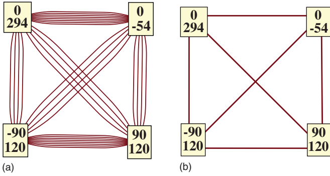
FIG. 1. (Color online) Wave numbers m, n are shown in the rectangles as upper and lower numbers. The smallest tridents cluster formed by eight symmetry generated solutions, two presentation forms are given: With multiedges (left-hand panel) and without multiedges (right-hand panel).
