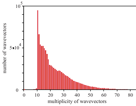
FIG. 9. (Color online) The multiplicities histogram for angle resonances.
