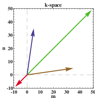
FIG. 3. (Color online) Wave vectors are shown which form first nonaxial trident (nonaxial trident with the smallest possible wave numbers m, n ).
